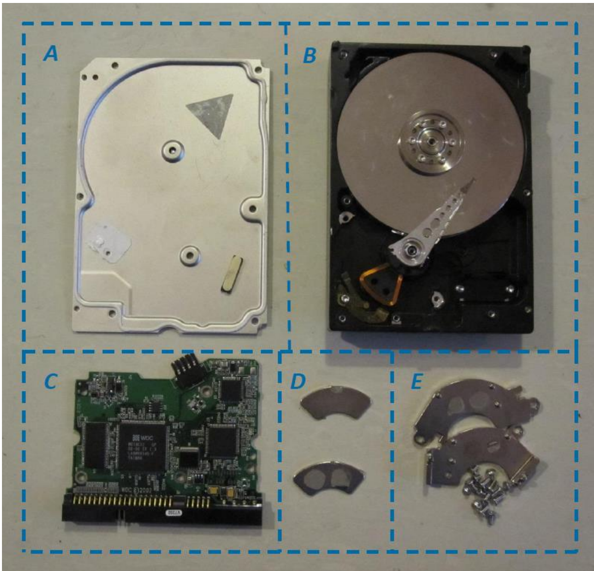
Picture 1-2: Dismantling depth of the hard disk drive dismantling trial (scenario 3): A: Lid; B: Case with platters and voice coil assembly; C: Printed wiring board; D: Magnets; E: Magnet shoes and other steel parts
